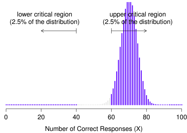
Sampling Distribution for X if \theta = .70
