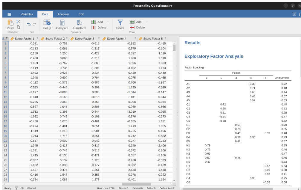
Figure 15.11: Data sheet view showing the five newly created factor score variables
