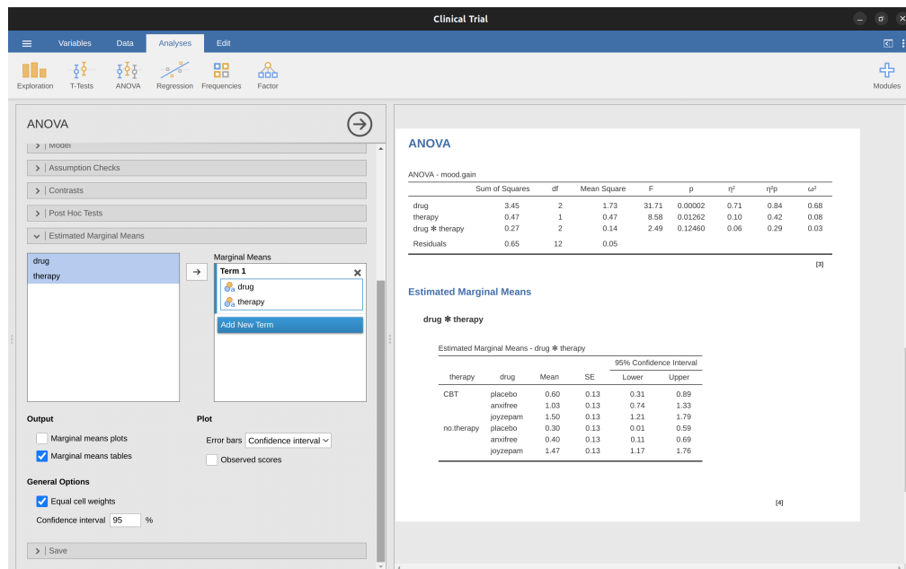
Figure 14.8: jamovi screenshot showing the marginal means for the saturated model, i.e. including the interaction component, with the clinical trial data set
