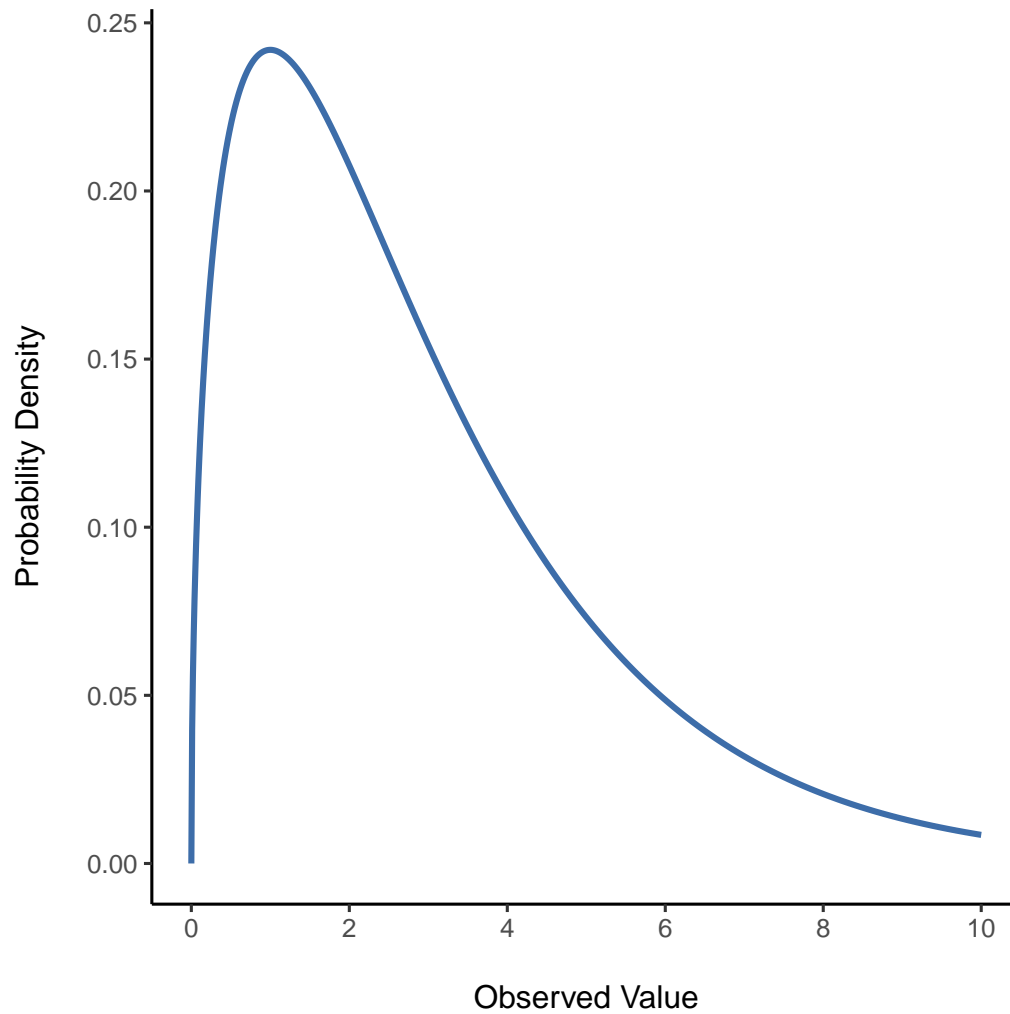
Figure 7.11: \chi^2 distribution with 3 degrees of freedom. Notice that the observed values must always be greater than zero, and that the distribution is pretty skewed. These are the key features of a chi-square distribution
