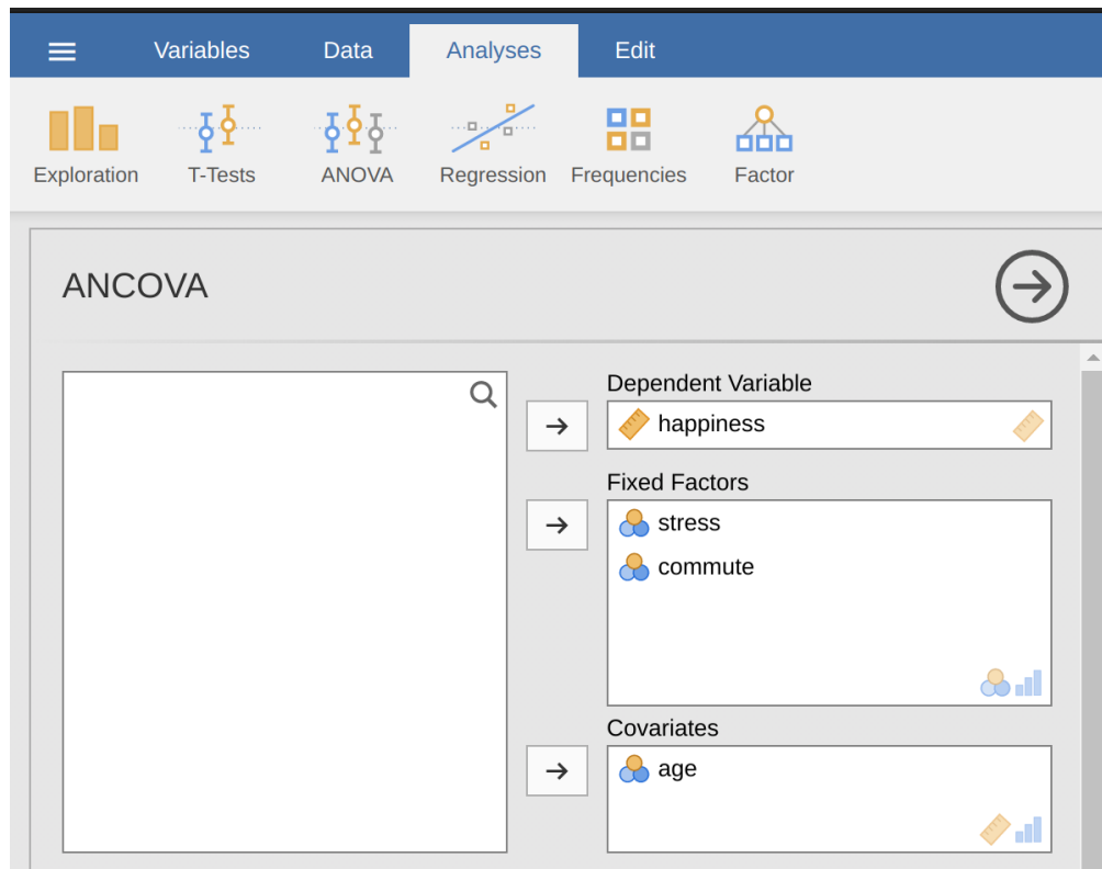
Figure 14.12: The jamovi ANCOVA analysis window
