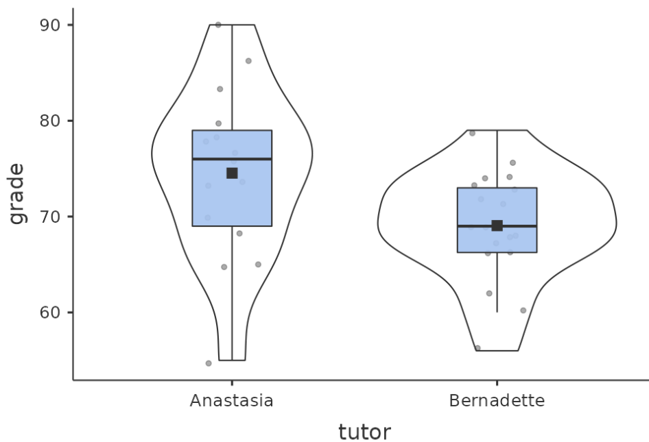
Figure 11.7: Box and violin plots showing the distribution of grades for students in Anastasia’s and Bernadette’s classes. Visually, these suggest that students in Anastasia’s class may be getting slightly better grades on average, though they also seem a bit more variable
