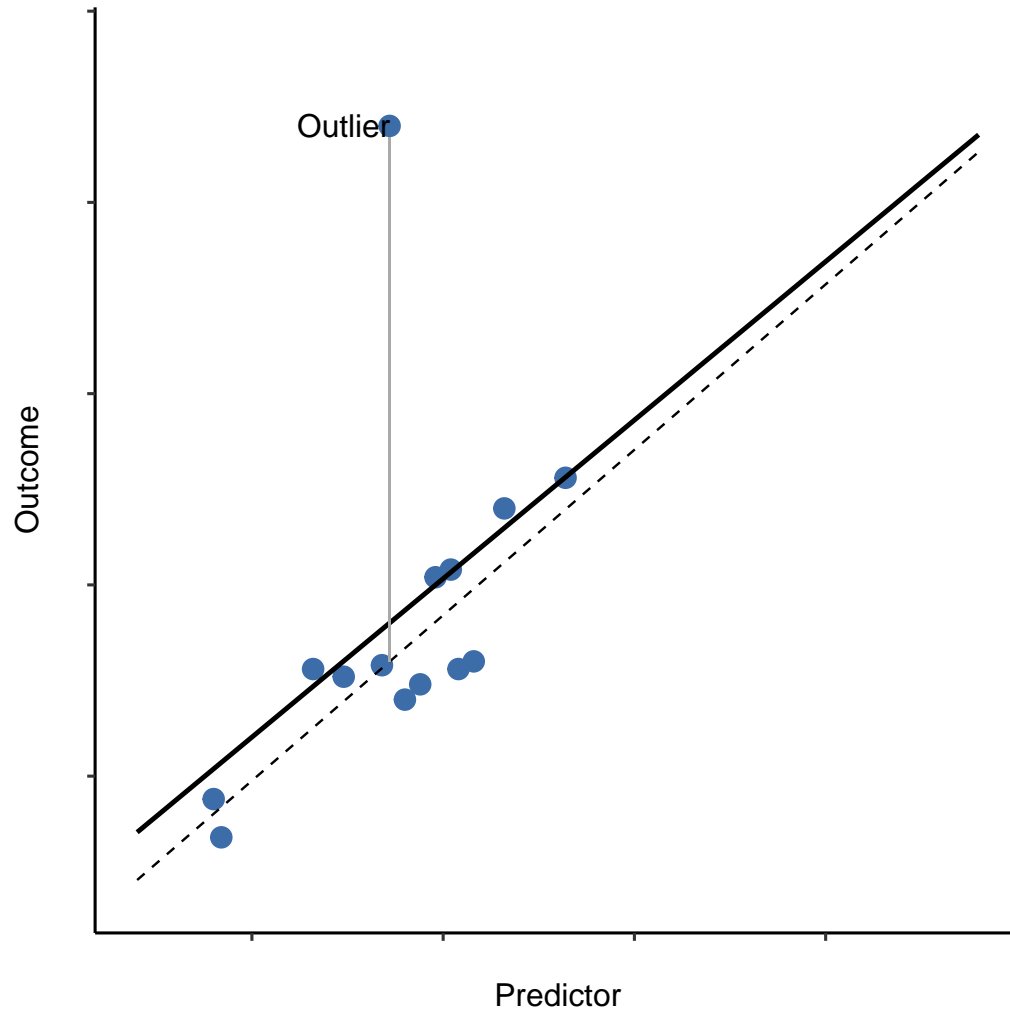
Figure 12.24: An illustration of outliers. The solid line shows the regression line with the anomalous outlier observation included. The dashed line plots the regression line estimated without the anomalous outlier observation included. The vertical line from the outlier point to the dashed regression line illustrates the large residual error for the outlier. The outlier has an unusual value on the outcome (y axis location) but not the predictor (x axis location), and lies a long way from the regression line
