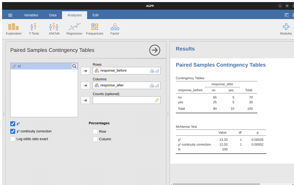
Figure 10.8: McNemar test output in jamovi
