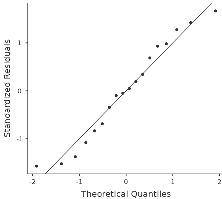
Figure 14.10: Checking assumptions in an ANOVA model
