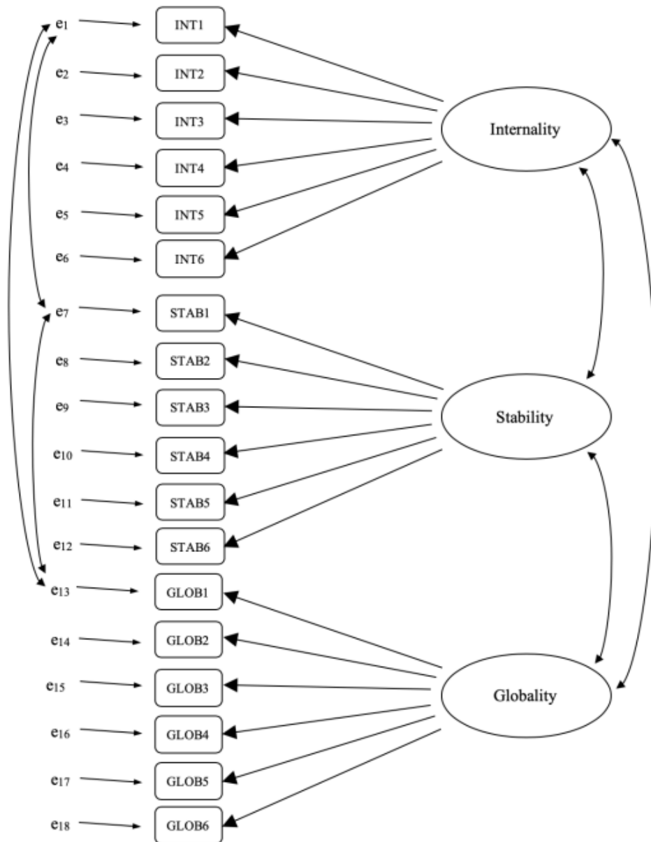
Figure 15.23: Final pre-specification of latent factor structure for the ASQ, including latent factor correlations, and shared method error term correlations for the observed variable INT1, STAB1 and GLOB1, in a CFA MTMM model. For clarity, other pre-specified error term correlations are not shown
