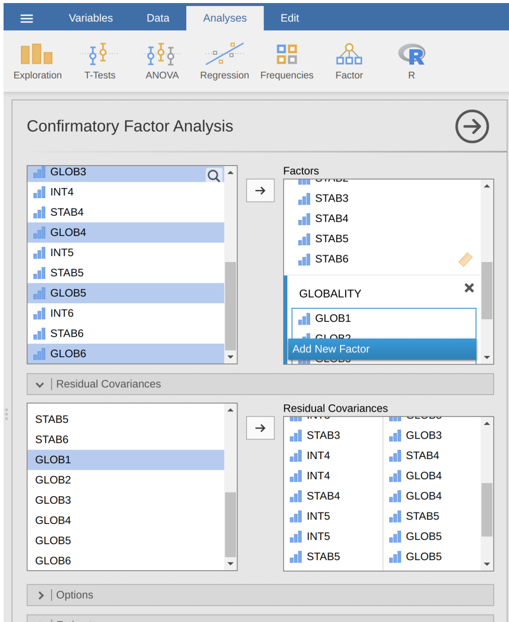
Figure 15.24: The jamovi CFA analysis window
