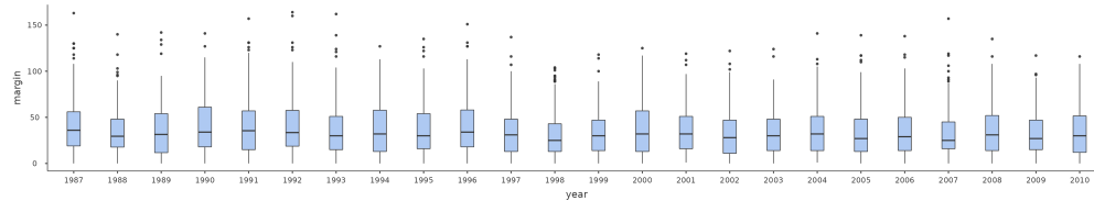
Figure 5.7: Multiple boxplots plotted in jamovi, for the margin by year variables
