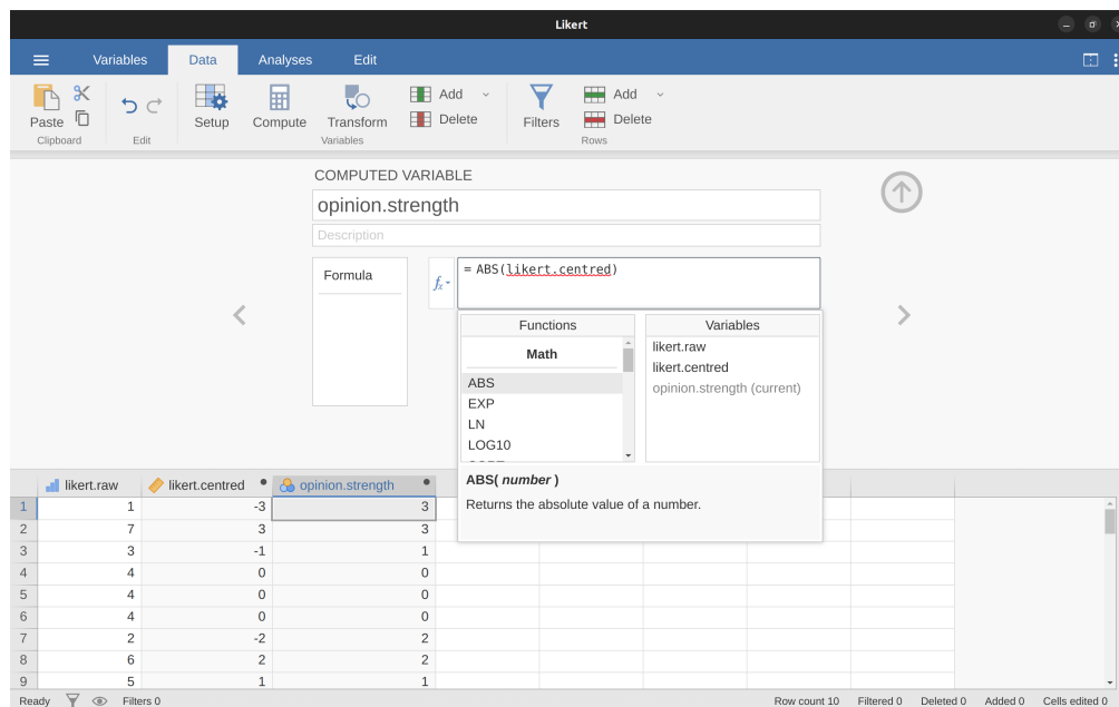
Figure 6.5: Using the f_x button to select functions and variables
