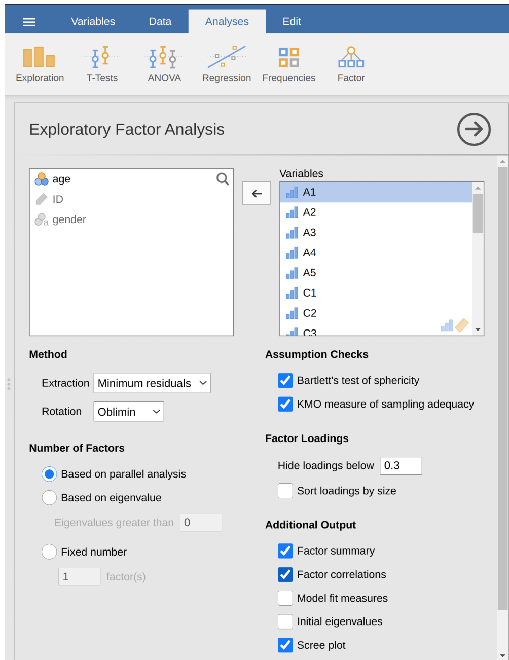
Figure 15.3: The jamovi EFA analysis window
