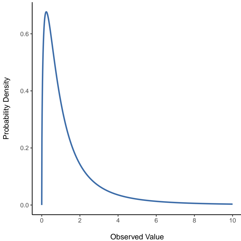
Figure 7.12: An F distribution with 3 and 5 degrees of freedom. Qualitatively speaking, it looks pretty similar to a chi-square distribution, but they're not quite the same in general
