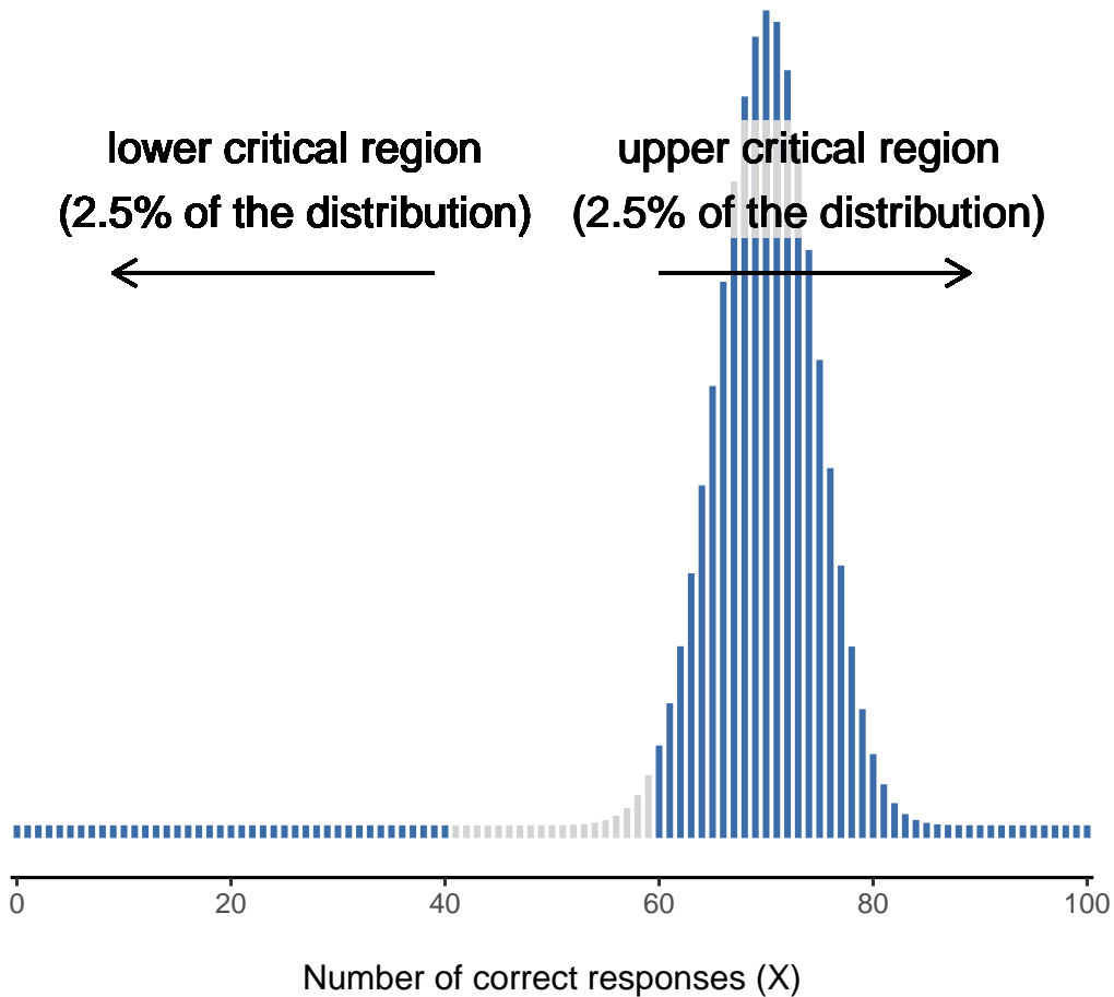
Figure 9.6: Sampling distribution under the alternative hypothesis for a population parameter value of \theta = 0.70 . Almost all of the distribution lies in the rejection region.
