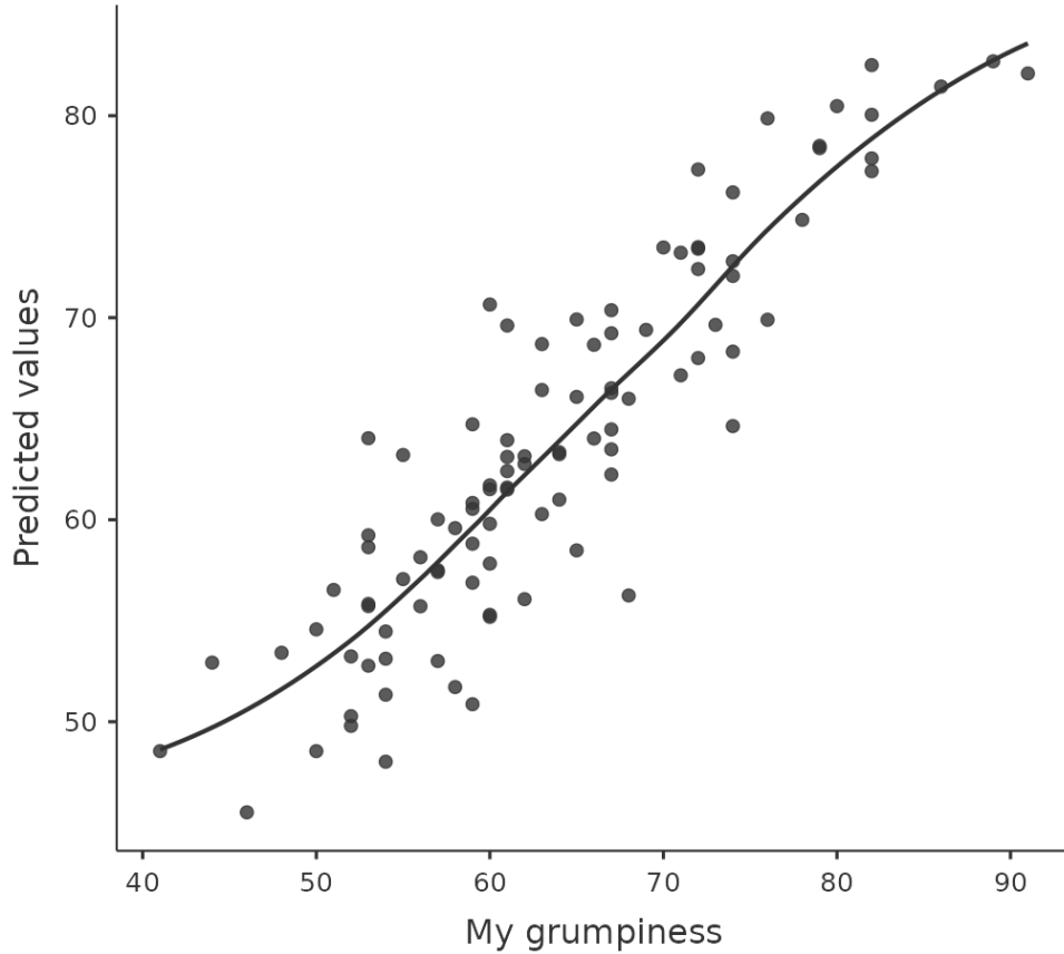
Figure 12.17: jamovi plot of the predicted values against the observed values of the outcome variable. A straight(-ish) line is what we're hoping to see here. This looks pretty good, suggesting that there's nothing grossly wrong
