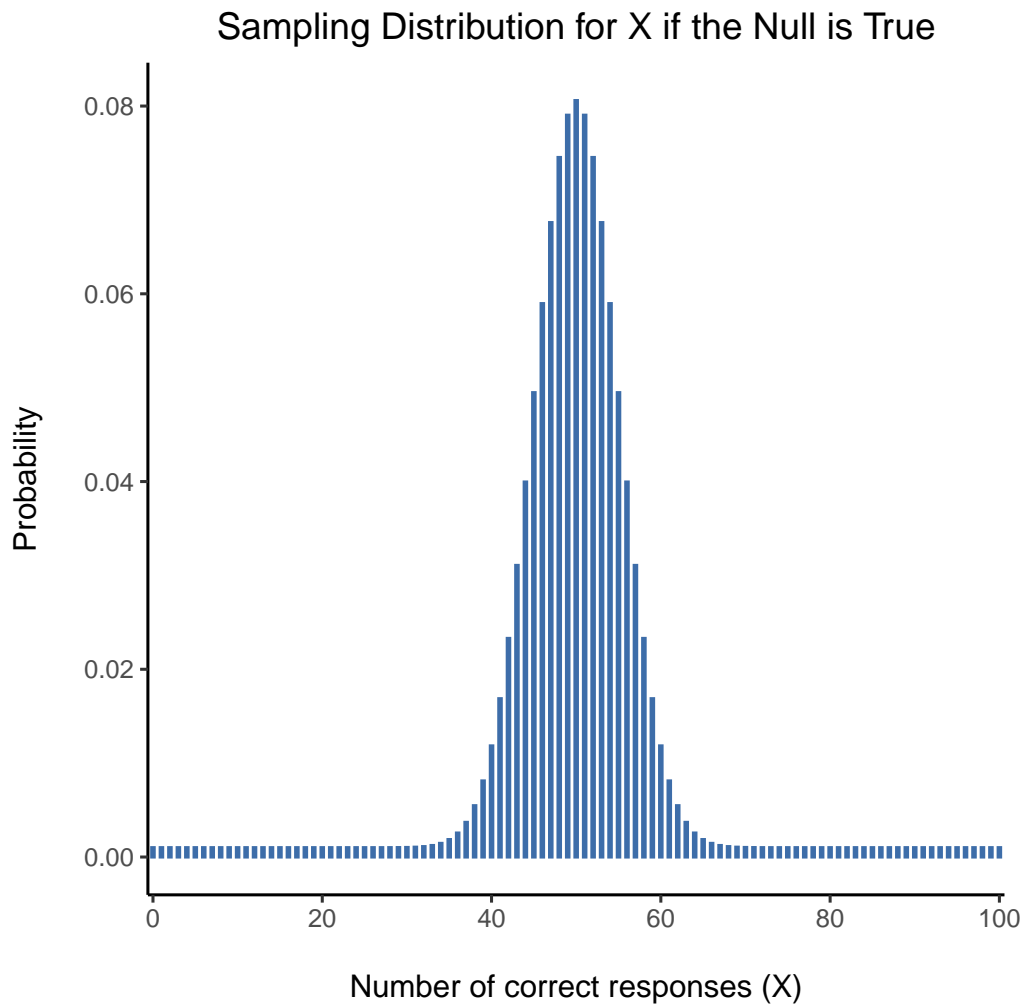
Figure 9.1: The sampling distribution for our test statistic X when the null hypothesis is true. For our ESP scenario this is a binomial distribution. Not surprisingly, since the null hypothesis says that the probability of a correct response is \theta = .5 , the sampling distribution says that the most likely value is 50 (out of 100) correct responses. Most of the probability mass lies between 40 and 60
