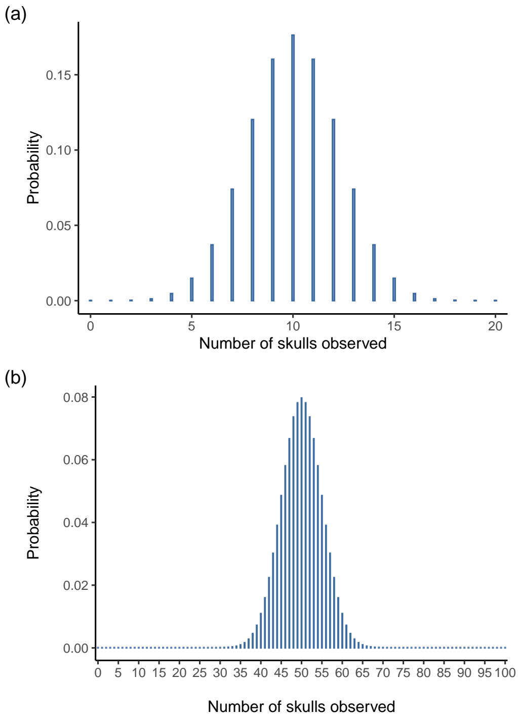
Figure 7.4: Two binomial distributions, involving a scenario in which I flip a fair coin so the underlying success probability is \theta = \frac{1}{2} . In panel (a), I flipped the coin N = 20 times. In panel (b) the coin was flipped N = 100 times
