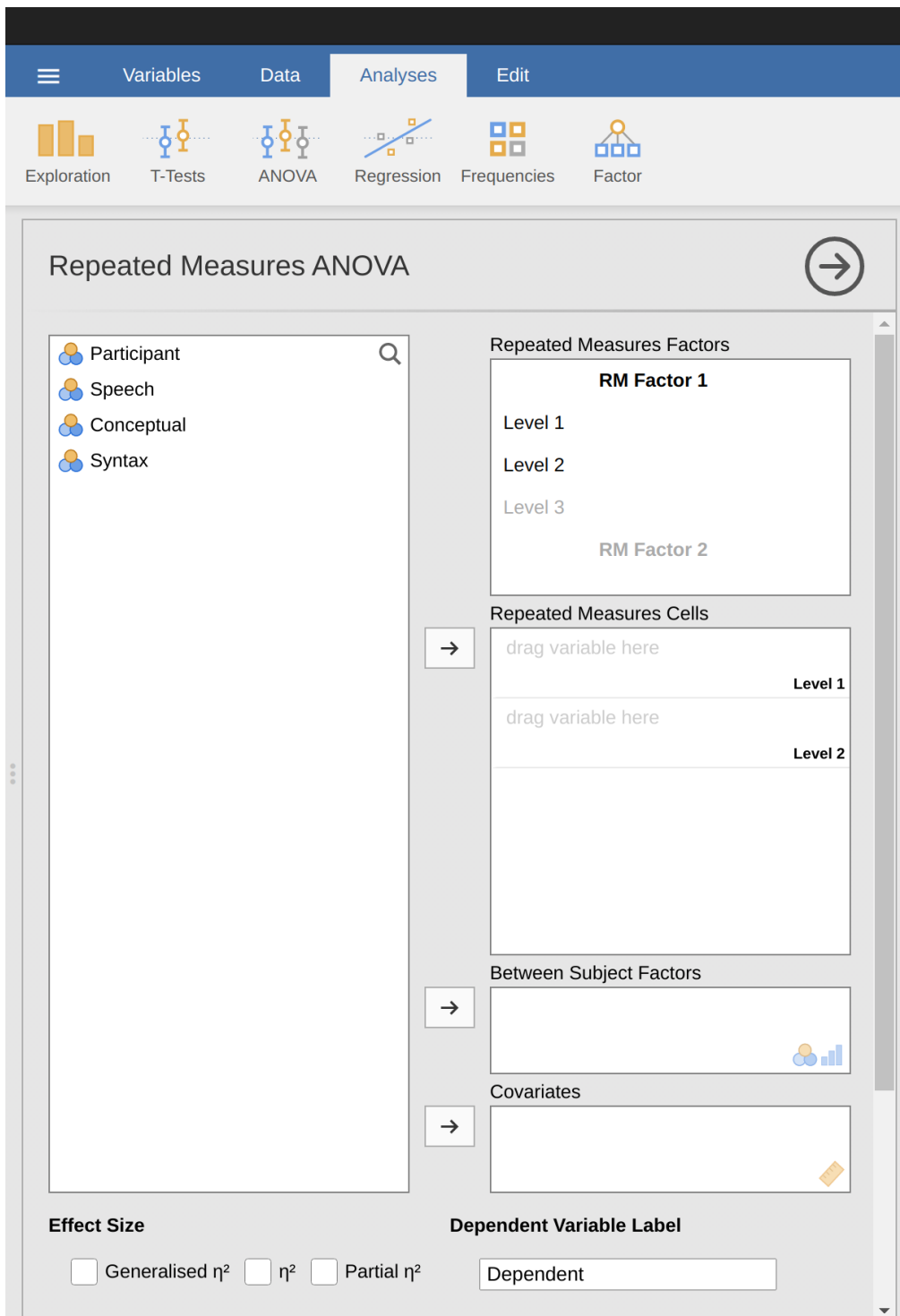
Figure 13.9: Repeated measures ANOVA dialog box in jamovi
