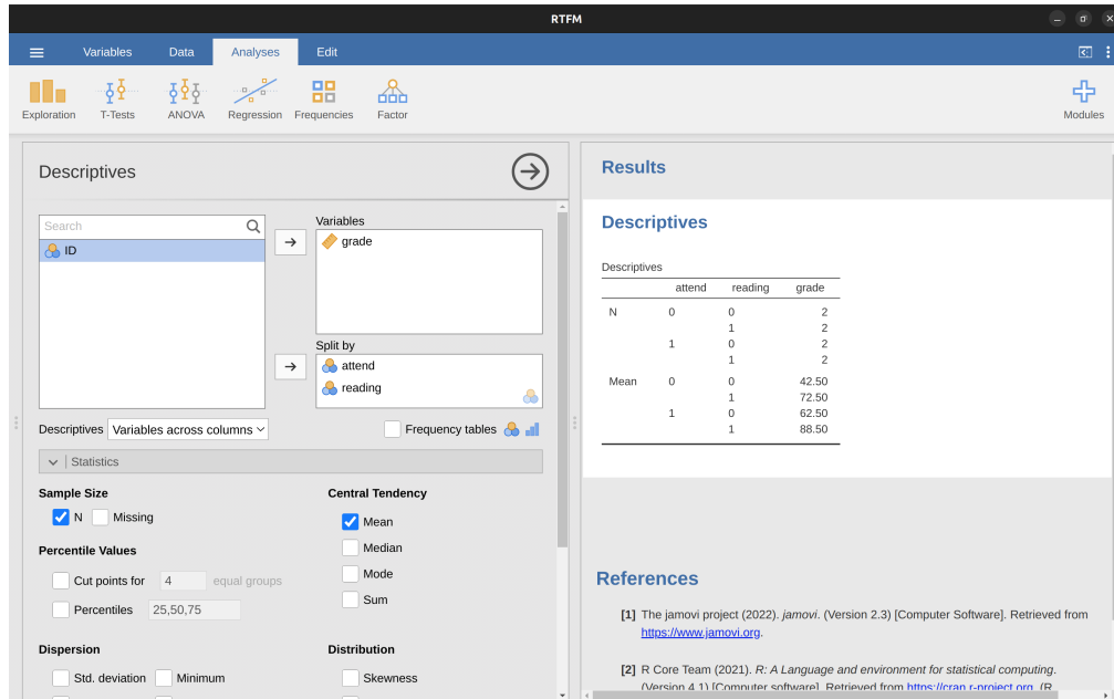
Figure 14.16: jamovi descriptives for the rtfm data set
