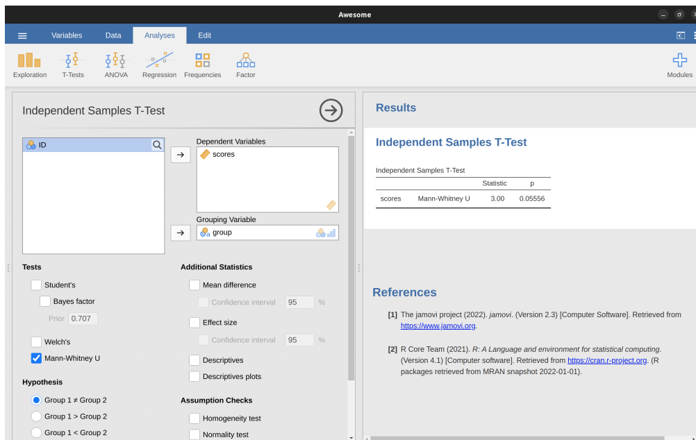
Figure 11.26: jamovi screen showing results for the Mann-Whitney U test
