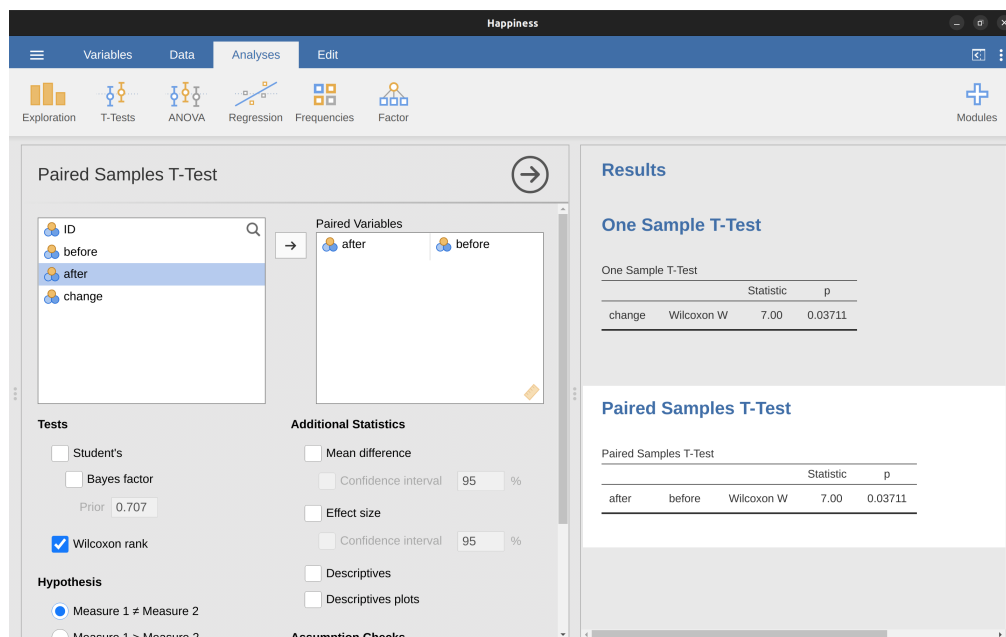
Figure 11.27: jamovi screen showing results for one sample and paired sample Wilcoxon nonparametric tests
