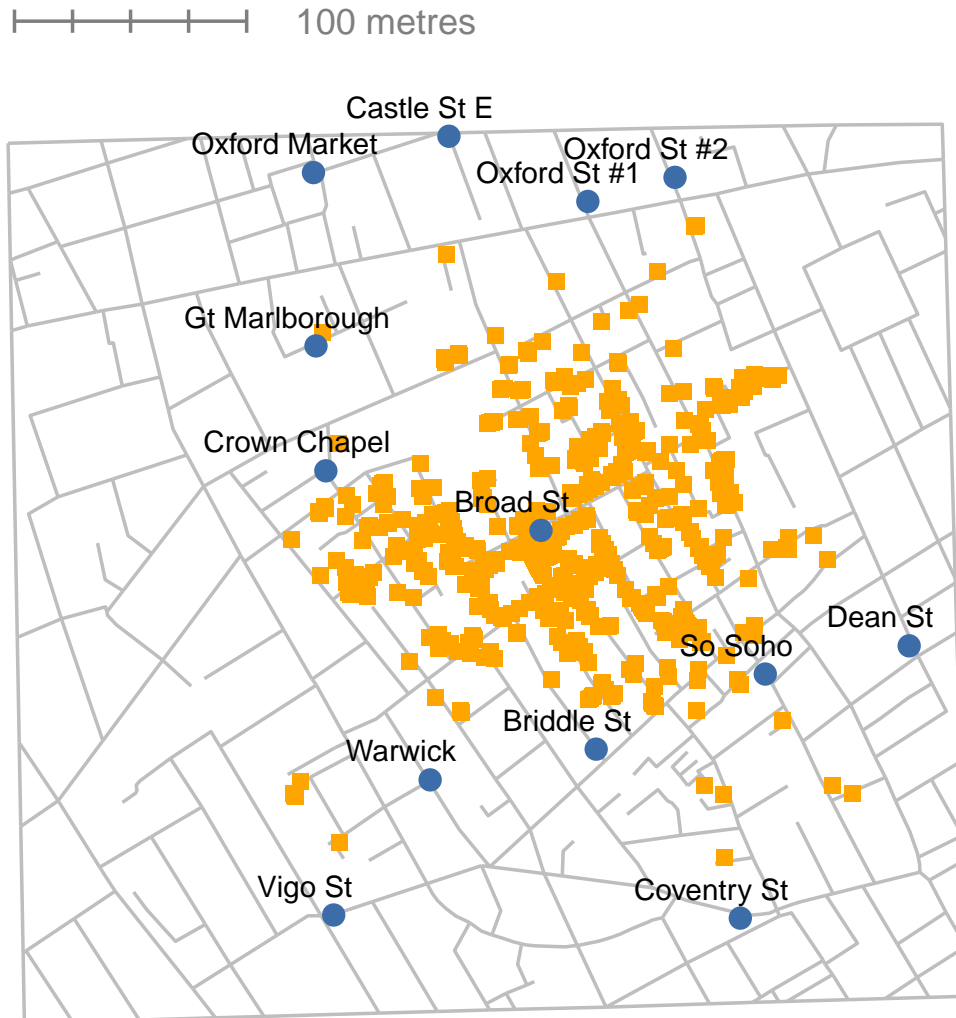
Figure 5.1: A stylised redrawing of John Snow's original cholera map. Each small orange square represents the location of a cholera death and each blue circle shows the location of a water pump. As the plot makes clear, the cholera outbreak is centred very closely on the Broad St pump
