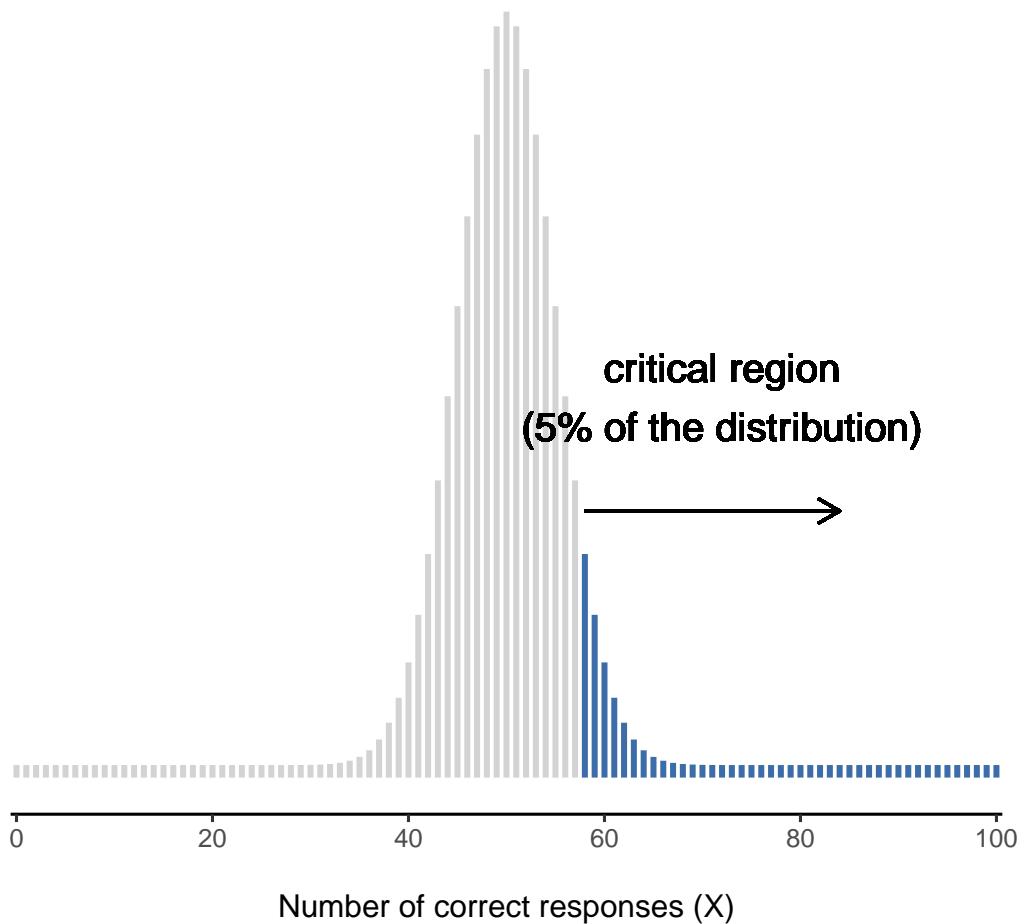
Figure 9.3: The critical region for a one sided test. In this case, the alternative hypothesis is that \theta \geq .5 so we would only reject the null hypothesis for large values of X . As a consequence, the critical region only covers the upper tail of the sampling distribution, specifically the upper 5% of the distribution. Contrast this to the two-sided version in Figure 9.2
