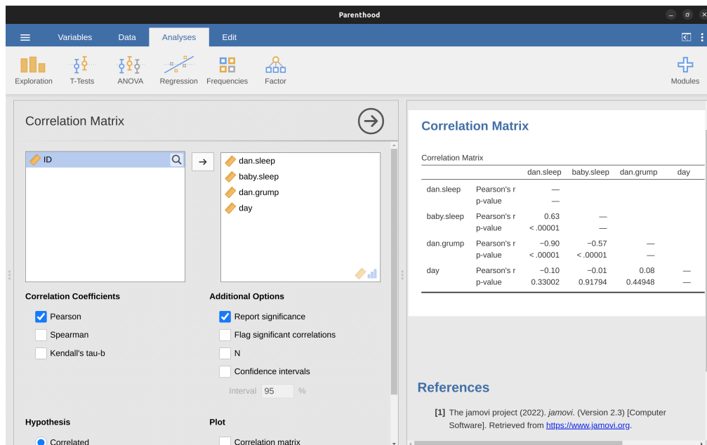
Figure 12.5: A jamovi screenshot showing correlations between variables in the parent-hood.csv file
