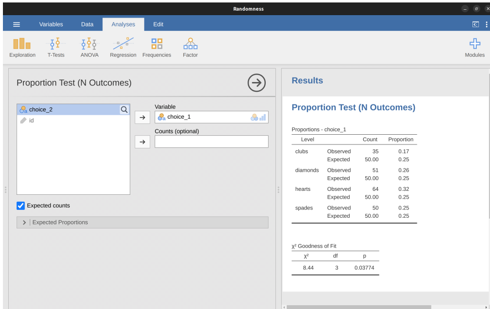
Figure 10.4: A \chi^2 One Sample Proportion Test in jamovi, with table showing both observed and expected frequencies and proportions
