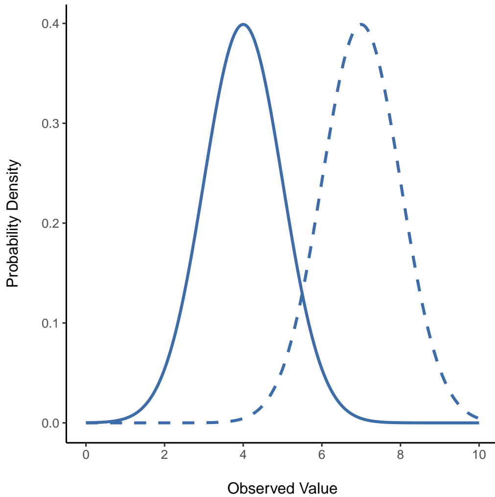
Figure 7.6: An illustration of what happens when you change the mean of a normal distribution. The solid line depicts a normal distribution with a mean of \mu = 4 . The dashed line shows a normal distribution with a mean of \mu = 7 . In both cases, the standard deviation is \sigma = 1 . Not surprisingly, the two distributions have the same shape, but the dashed line is shifted to the right
