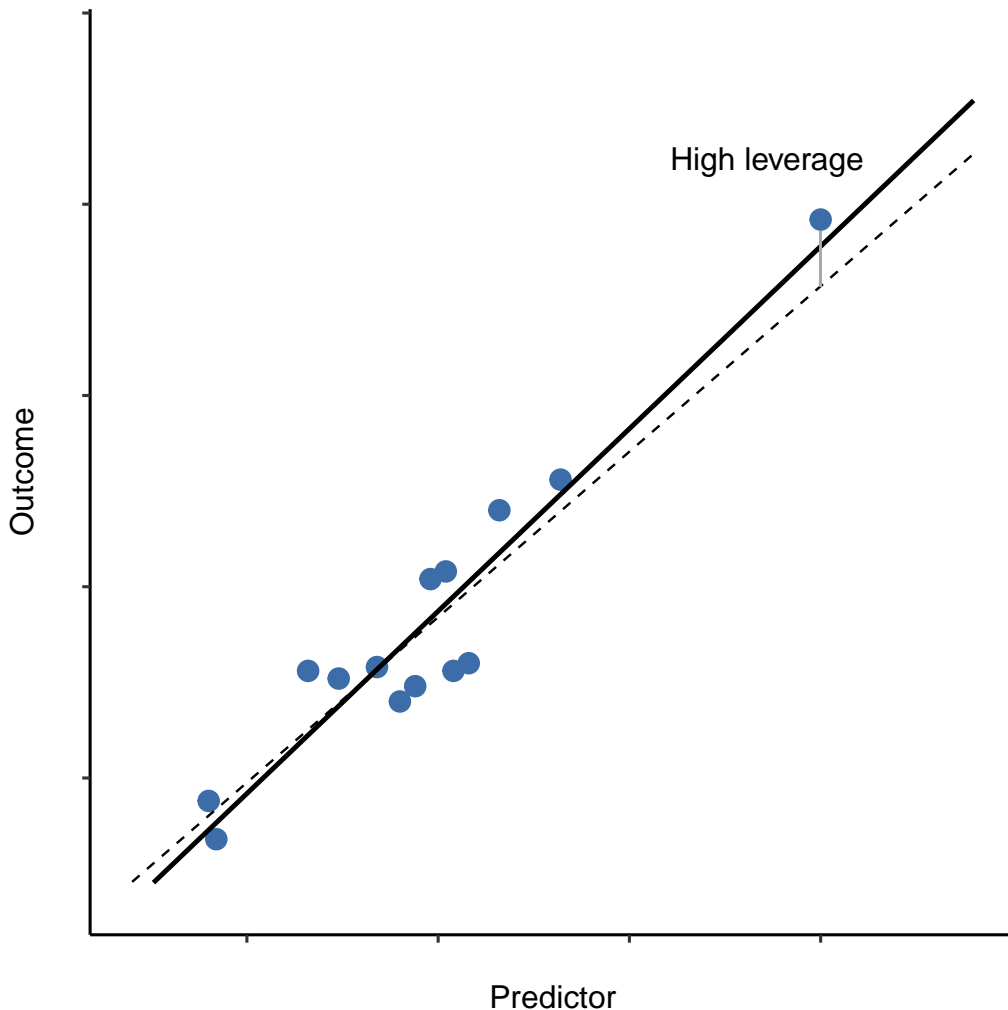
Figure 12.25: An illustration of high leverage points. The anomalous observation in this case is unusual both in terms of the predictor (x axis) and the outcome (y axis), but this unusualness is highly consistent with the pattern of correlations that exists among the other observations. The observation falls very close to the regression line and does not distort it by very much
