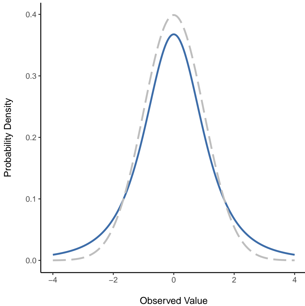
Figure 7.10: A t distribution with 3 degrees of freedom (solid line). It looks similar to a normal distribution, but it's not quite the same. For comparison purposes I've plotted a standard normal distribution as the dashed line
