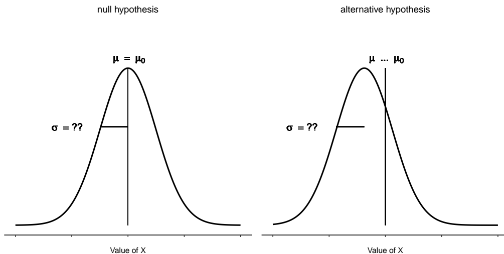
Figure 11.4: Graphical illustration of the null and alternative hypotheses assumed by the (two sided) one sample t-test. Note the similarity to the z-test (Figure 11.2). The null hypothesis is that the population mean \mu is equal to some specified value \mu_0 , and the alternative hypothesis is that it is not. Like the z-test, we assume that the data are normally distributed, but we do not assume that the population standard deviation \sigma is known in advance
