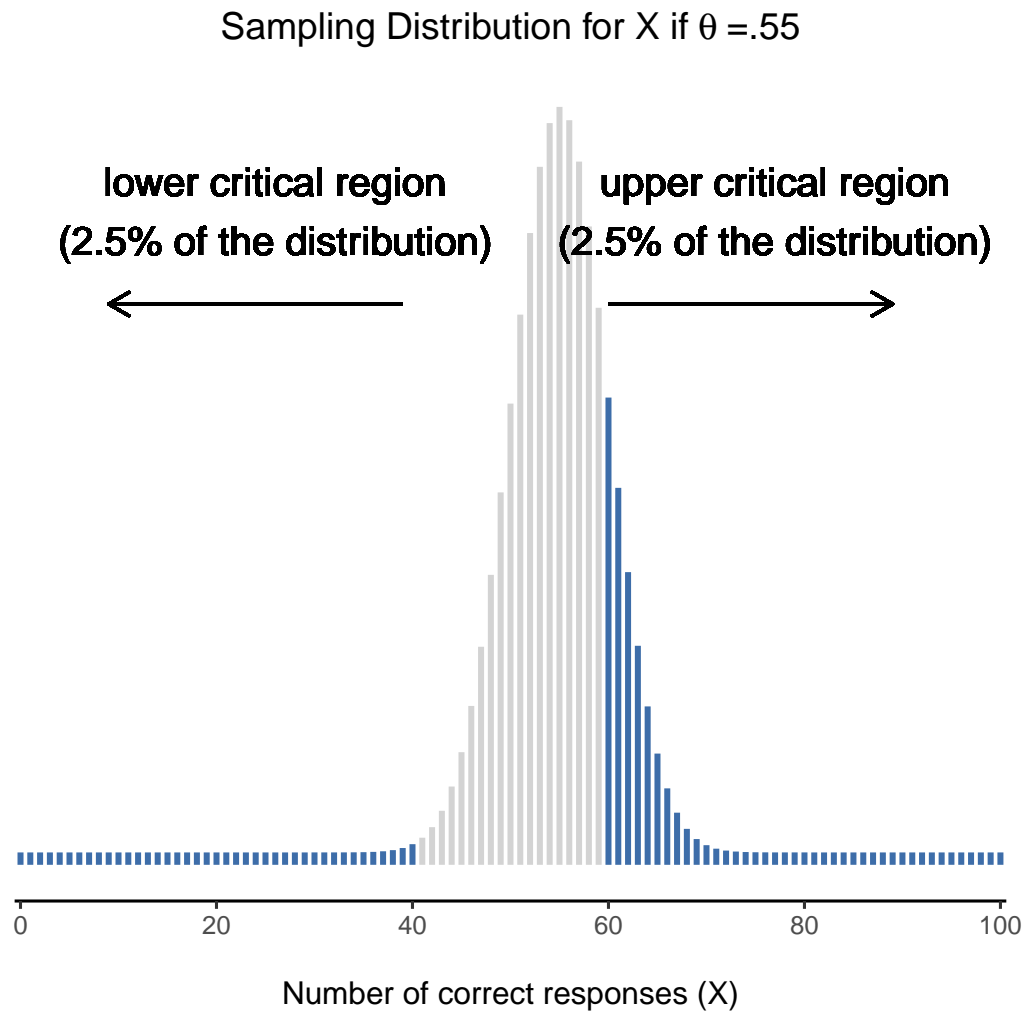
Figure 9.5: Sampling distribution under the alternative hypothesis for a population parameter value of \theta = 0.55 . A reasonable proportion of the distribution lies in the rejection region
