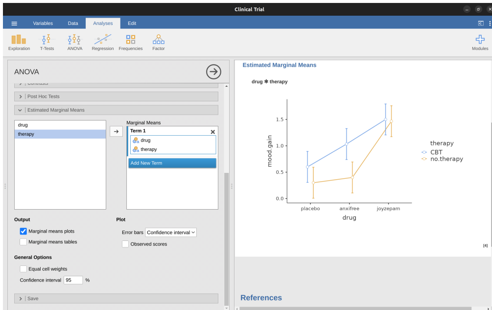
Figure 14.6: jamovi screen showing how to generate a descriptive interaction plot in ANOVA using the clinical trial data
