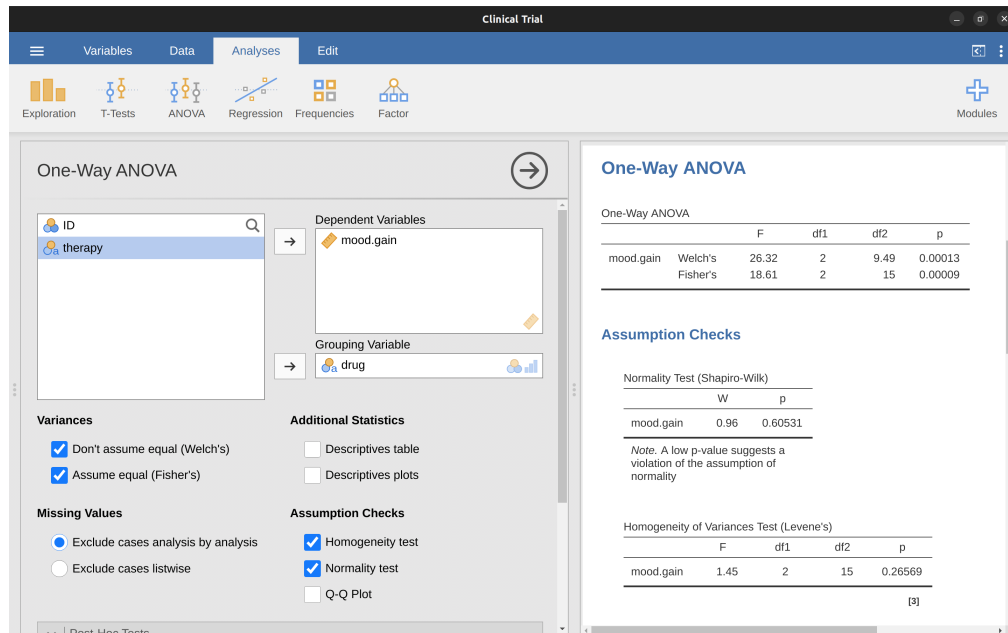
Figure 13.6: Welch's test as part of the One Way ANOVA analysis in jamovi
