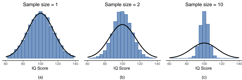
Figure 8.8: An illustration of the how sampling distribution of the mean depends on sample size. In each panel I generated 10,000 samples of IQ data and calculated the mean IQ observed within each of these data sets. The histograms in these plots show the distribution of these means (i.e., the sampling distribution of the mean). Each individual IQ score was drawn from a normal distribution with mean 100 and standard deviation 15, which is shown as the solid black line. In panel (a), each data set contained only a single observation, so the mean of each sample is just one person's IQ score. As a consequence, the sampling distribution of the mean is of course identical to the population distribution of IQ scores. However, when we raise the sample size to 2 the mean of any one sample tends to be closer to the population mean than any one person's IQ score, and so the histogram (i.e., the sampling distribution) is a bit narrower than the population distribution. By the time we raise the sample size to 10 (panel (c)), we can see that the distribution of sample means tend to be fairly tightly clustered around the true population mean
