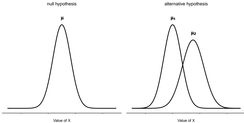
Figure 11.10: Graphical illustration of the null and alternative hypotheses assumed by the Welch t-test. Like the Student test (Figure 11.9) we assume that both samples are drawn from a normal population; but the alternative hypothesis no longer requires the two populations to have equal variance
