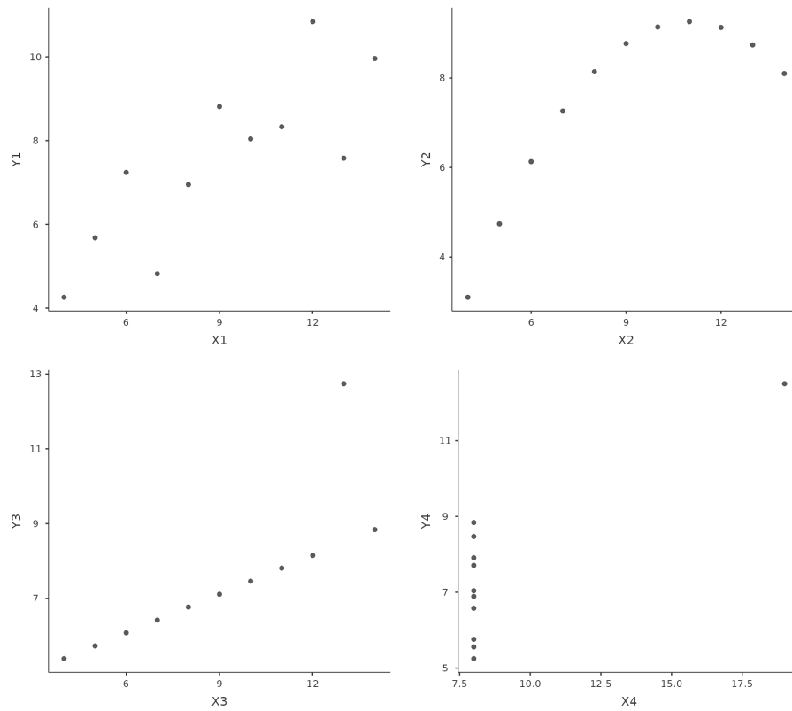
Figure 12.6: Anscombe's quartet scatterplots in jamovi. All four of these data sets have a Pearson correlation of r = .816 , but they are qualitatively different from one another
