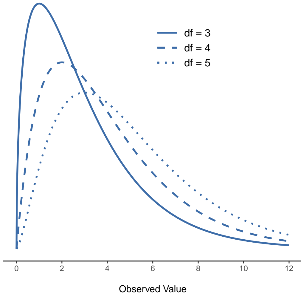
Figure 10.1: \chi^2 (chi-square) distributions with different values for the 'degrees of freedom'
