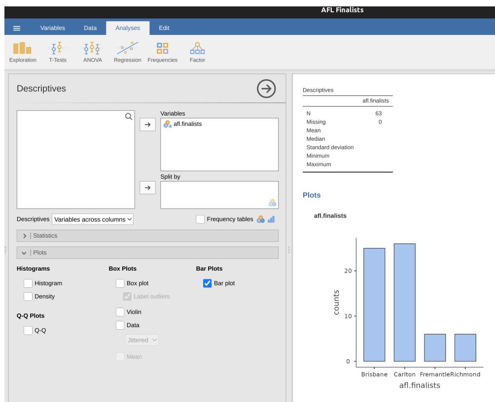
Figure 5.11: Filtering to include just four AFL teams, and drawing a bar plot in jamovi
