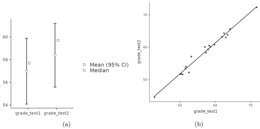
Figure 11.13: Mean grade for test 1 and test 2, with associated 95% confidence intervals (a). Scatterplot showing the individual grades for test 1 and test 2 (b).
