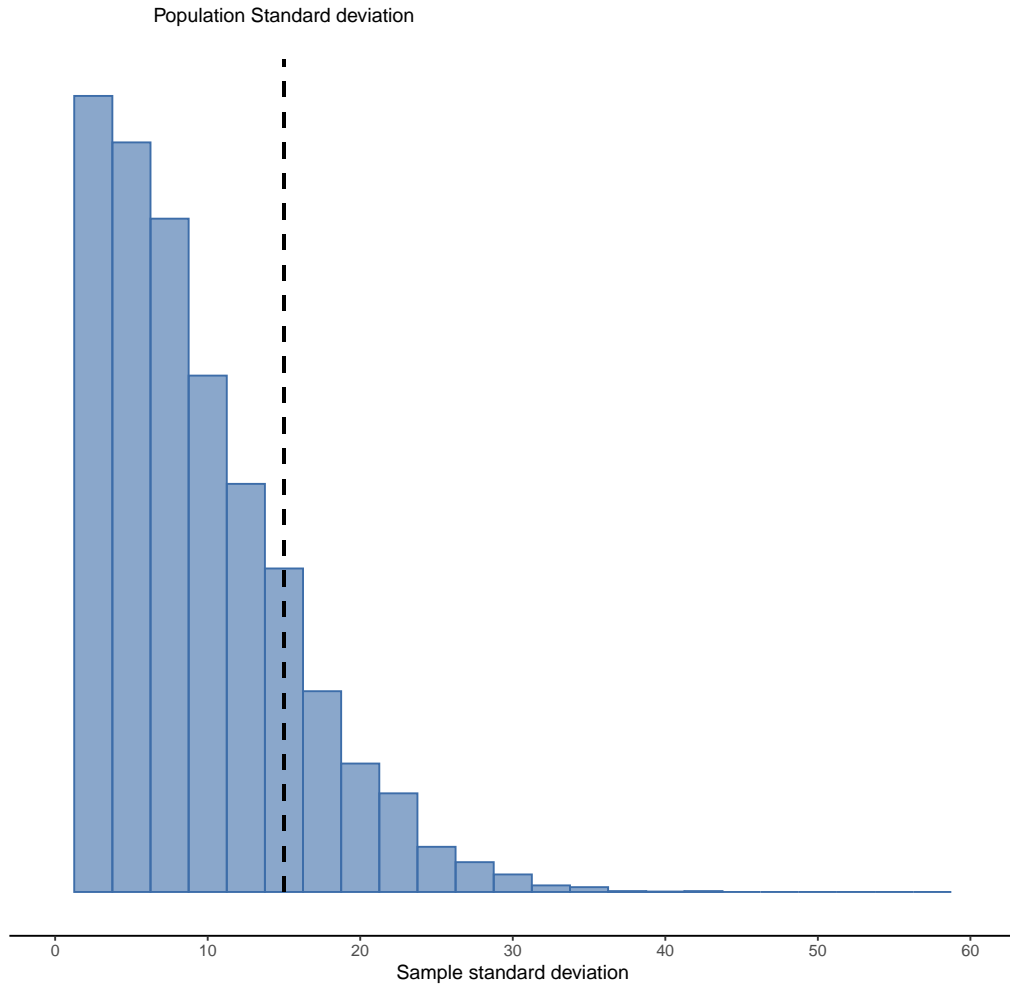
Figure 8.10: The sampling distribution of the sample standard deviation for a ‘two IQ scores’ experiment. The true population standard deviation is 15 (dashed line), but as you can see from the histogram the vast majority of experiments will produce a much smaller sample standard deviation than this. On average, this experiment would produce an estimated standard deviation of only 8.4, well below the true value! In other words, the sample standard deviation is a biased estimate of the population standard deviation
