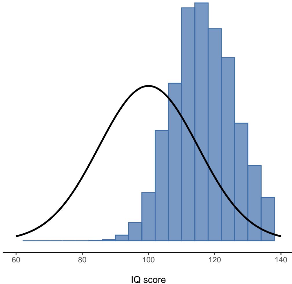
Figure 8.7: The sampling distribution of the maximum for the ‘five IQ scores experiment’. If you sample 5 people at random and select the one with the highest IQ score you’ll probably see someone with an IQ between 100 and 140
