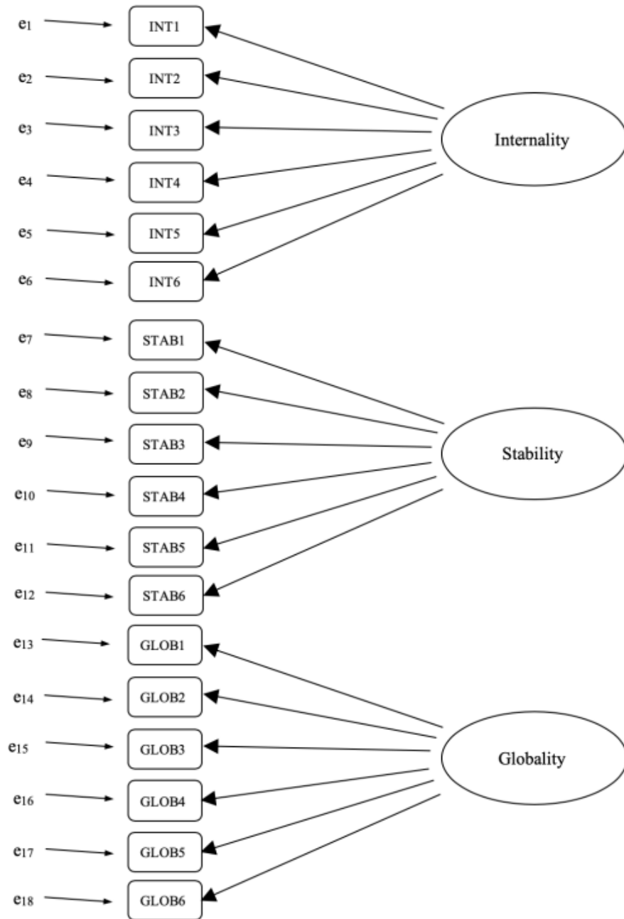
Figure 15.22: Initial pre-specification of latent factor structure for the ASQ
