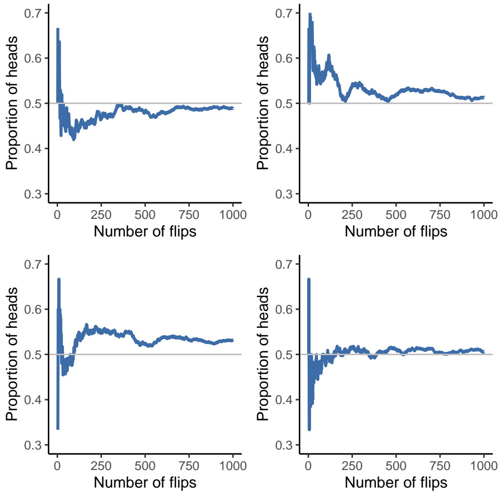
Figure 7.1: An illustration of how frequentist probability works. If you flip a fair coin over and over again the proportion of heads that you've seen eventually settles down and converges to the true probability of 0.5. Each panel shows four different simulated experiments. In each case we pretend we flipped a coin 1000 times and kept track of the proportion of flips that were heads as we went along. Although none of these sequences actually ended up with an exact value of .5, if we'd extended the experiment for an infinite number of coin flips they would have
