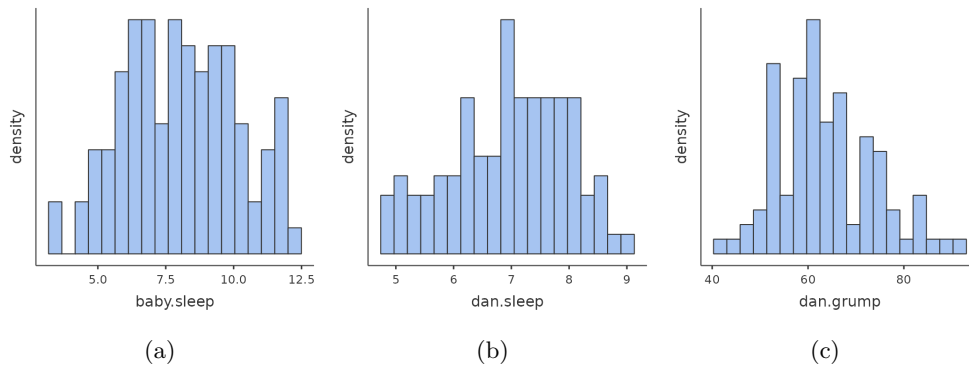
Figure 12.1: Histograms from jamovi for the three interesting variables in the parenthood data set
