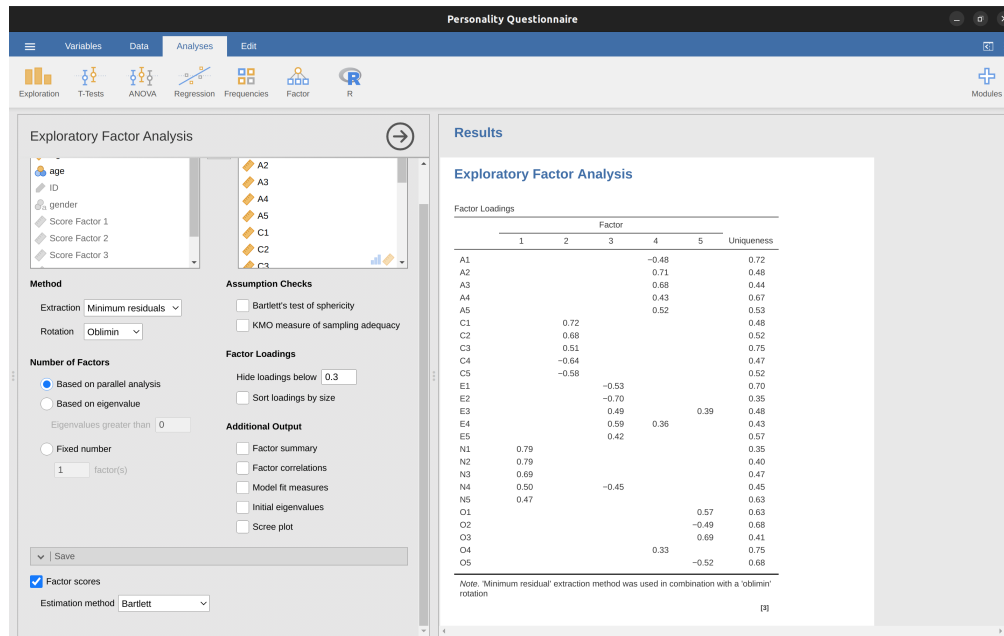
Figure 15.10: jamovi option for factor scores for the five factor solution, using the ‘Bartlett’ optimal weighting method
