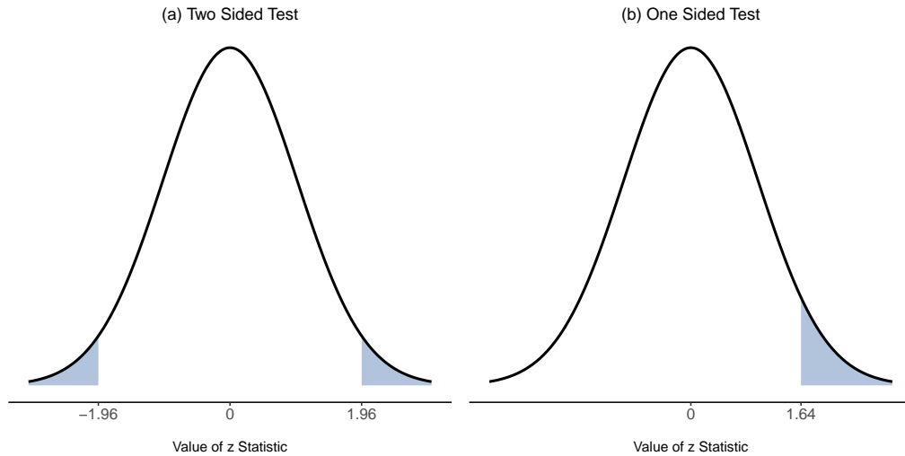
Figure 11.3: Rejection regions for the two-sided z-test (panel (a)) and the one-sided z-test (panel (b))
