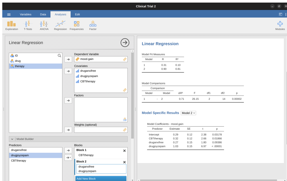
Figure 14.22: Model comparison in jamovi regression, null model 1 vs. contrasts model 2
