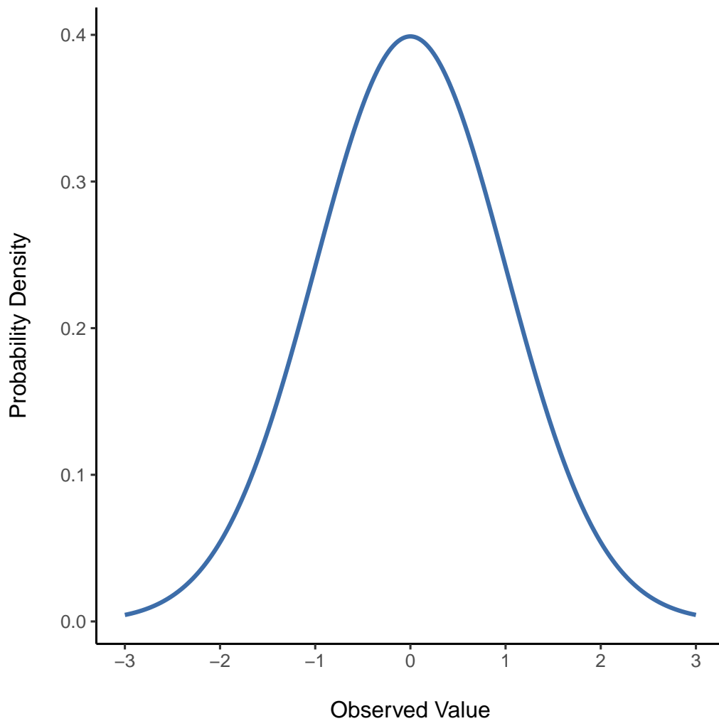
Figure 7.5: The normal distribution with mean \mu = 0 and standard deviation \sigma = 1 . The x-axis corresponds to the value of some variable, and the y-axis tells us something about how likely we are to observe that value. However, notice that the y-axis is labelled Probability Density and not Probability . There is a subtle and somewhat frustrating characteristic of continuous distributions that makes the y axis behave a bit oddly - the height of the curve here isn't actually the probability of observing a particular x value. On the other hand, it is true that the heights of the curve tells you which x values are more likely (the higher ones!). (see Probability density section for all the annoying details)
