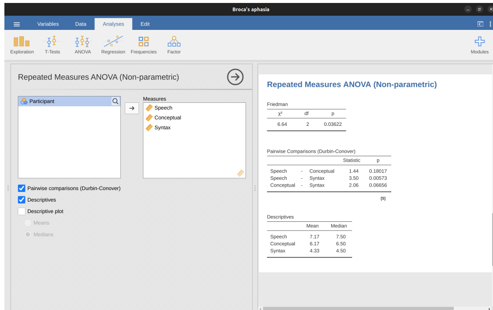
Figure 13.14: The ‘Repeated Measures ANOVA (Non-parametric)’ dialogue box and results in jamovi
