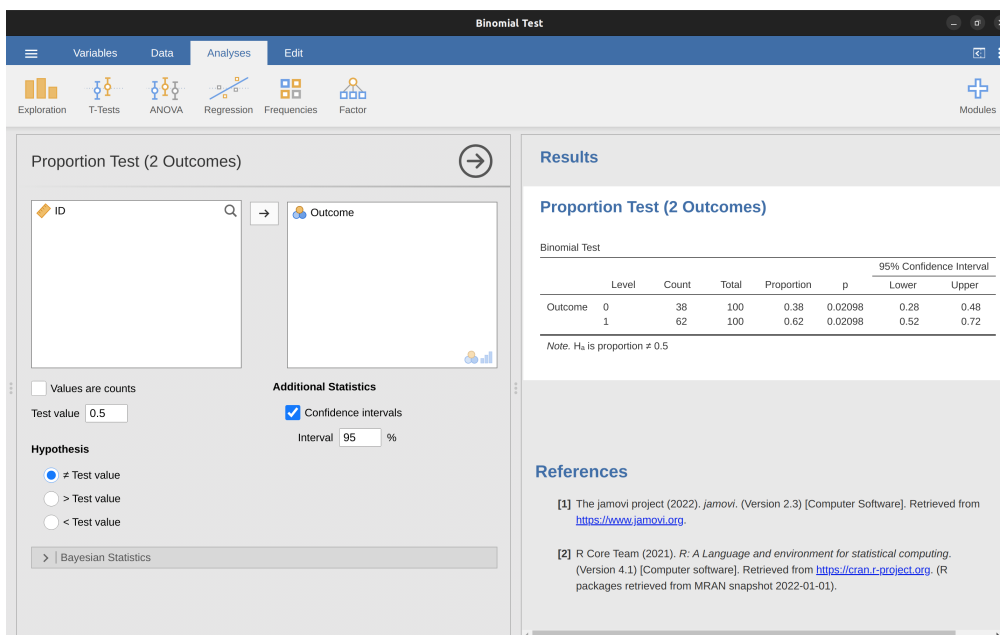
Figure 9.4: Binomial test analysis and results in jamovi
