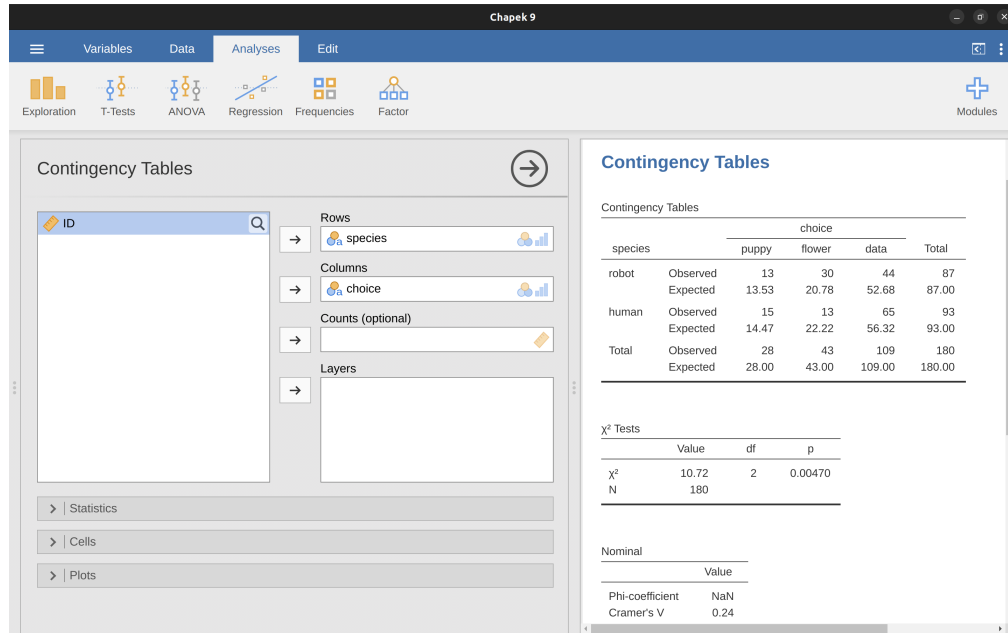
Figure 10.6: Independent samples \chi^2 test in jamovi using the Chapek 9 data
