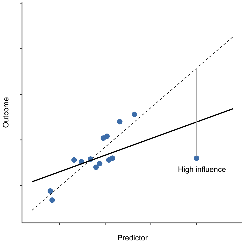
Figure 12.26: An illustration of high influence points. In this case, the anomalous observation is highly unusual on the predictor variable (x axis), and falls a long way from the regression line. As a consequence, the regression line is highly distorted, even though (in this case) the anomalous observation is entirely typical in terms of the outcome variable (y axis)
