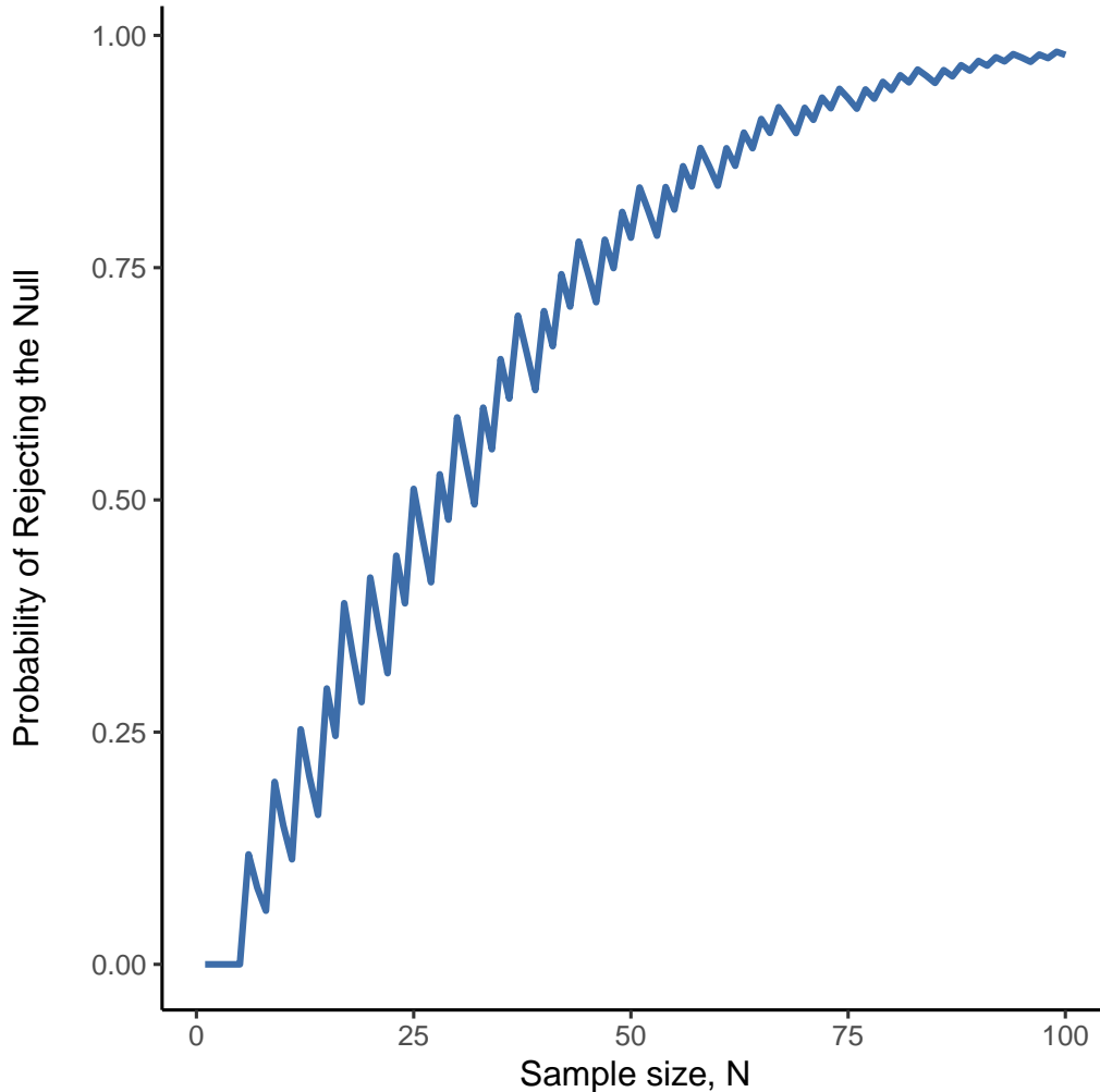
Figure 9.8: The power of our test plotted as a function of the sample size N . In this case, the true value of \theta is 0.7 but the null hypothesis is that \theta = 0.5 . Overall, larger N means greater power. (The small zig-zags in this function occur because of some odd interactions between \theta , \alpha and the fact that the binomial distribution is discrete, it doesn't matter for any serious purpose)
