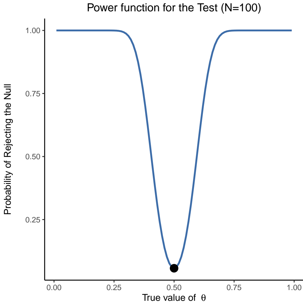
Figure 9.7: The probability that we will reject the null hypothesis, plotted as a function of the true value of \theta . Obviously, the test is more powerful (greater chance of correct rejection) if the true value of \theta is very different from the value that the null hypothesis specifies (i.e., \theta = .5 ). Notice that when \theta actually is equal to .5 (plotted as a black dot), the null hypothesis is in fact true and rejecting the null hypothesis in this instance would be a Type I error
