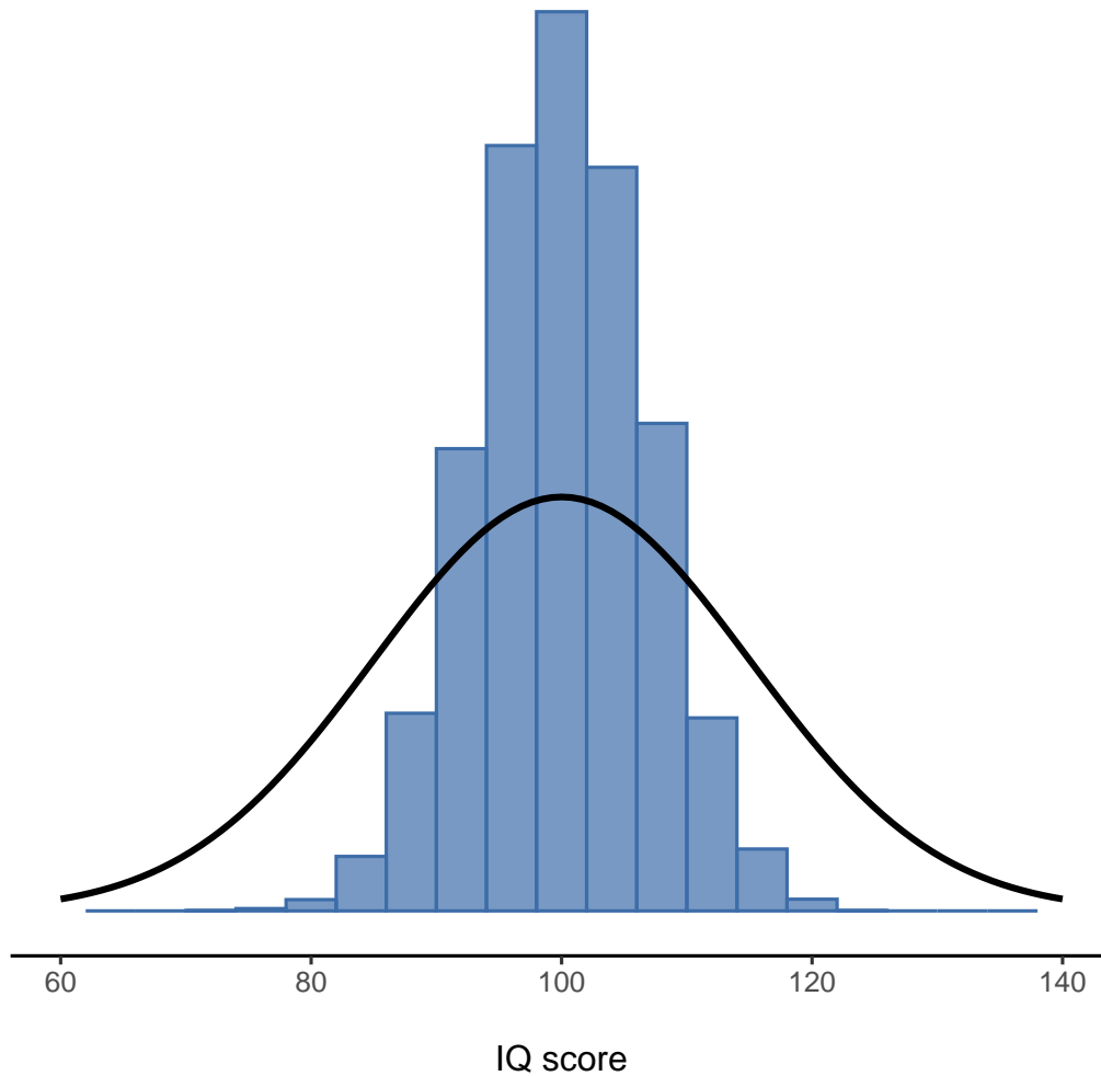
Figure 8.6: The sampling distribution of the mean for the ‘five IQ scores experiment’. If you sample 5 people at random and calculate their average IQ you’ll almost certainly get a number between 80 and 120, even though there are quite a lot of individuals who have IQs above 120 or below 80. For comparison, the black line plots the population distribution of IQ scores
