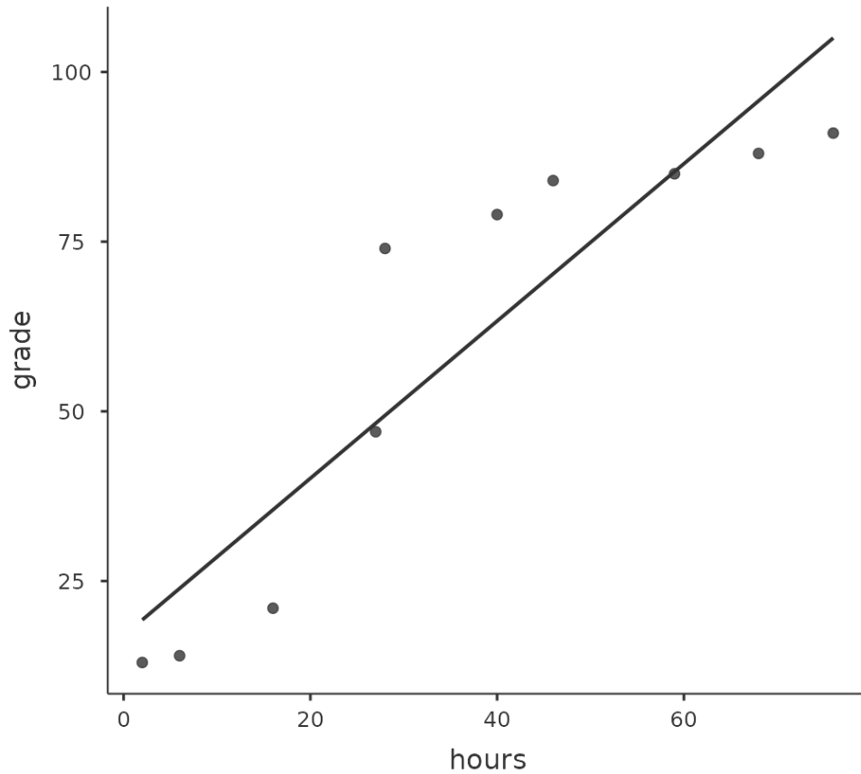
Figure 12.7: The relationship between hours worked and grade received for a toy data set consisting of only 10 students (each dot corresponds to one student). The line through the middle shows the linear relationship between the two variables. This produces a strong Pearson correlation of r = .91 . However, the interesting thing to note here is that there's actually a perfect monotonic relationship between the two variables. In this toy example, increasing the hours worked always increases the grade received, as illustrated by the solid line. This is reflected in a Spearman correlation of \rho = 1 . With such a small data set, however, it's an open question as to which version better describes the actual relationship involved
