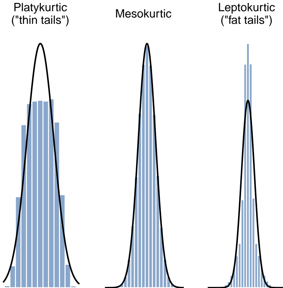
Figure 4.12: An illustration of kurtosis. On the left, we have a ‘platykurtic’ distribution (kurtosis = -0.95 ) meaning that the distribution has ‘thin’ or flat tails. In the middle we have a ‘mesokurtic’ distribution (kurtosis is almost exactly 0) which means that the tails are neither thin or fat. Finally, on the right, we have a ‘leptokurtic’ distribution (kurtosis = 2.12 ) indicating that the distribution has ‘fat’ tails. Note that kurtosis is measured with respect to a normal curve (black line)
