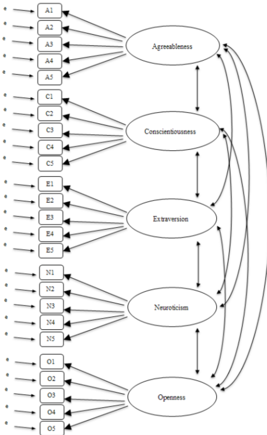
Figure 15.13: Initial pre-specification of latent factor structure for the five factor personality scales, for use in CFA
