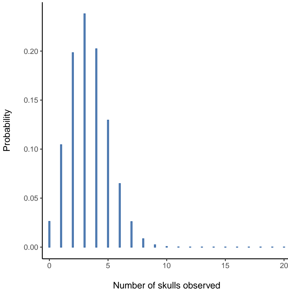
Figure 7.3: The binomial distribution with size parameter of N = 20 and an underlying success probability of \theta = \frac{1}{6} . Each vertical bar depicts the probability of one specific outcome (i.e., one possible value of X ). Because this is a probability distribution, each of the probabilities must be a number between 0 and 1, and the heights of the bars must sum to 1 as well
