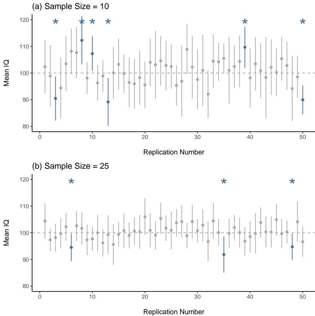
Figure 8.12: 95% confidence intervals. The top panel (a) shows 50 simulated replications of an experiment in which we measure the IQs of 10 people. The dot marks the location of the sample mean and the line shows the 95% confidence interval. Most of the 50 confidence intervals do contain the true mean (i.e., 100), but a few - in blue and marked with asterisks - do not. The lower graph (panel b) shows a similar simulation, but this time we simulate replications of an experiment that measures the IQs of 25 people
