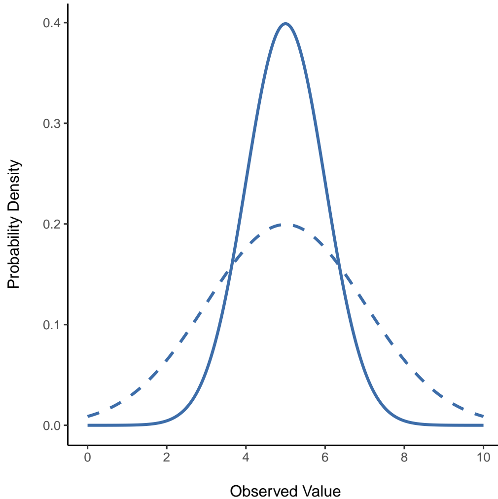
Figure 7.7: An illustration of what happens when you change the the standard deviation of a normal distribution. Both distributions plotted in this figure have a mean of \mu = 5 , but they have different standard deviations. The solid line plots a distribution with standard deviation \sigma = 1 , and the dashed line shows a distribution with standard deviation \sigma = 2 . As a consequence, both distributions are ‘centred’ on the same spot, but the dashed line is wider than the solid one
