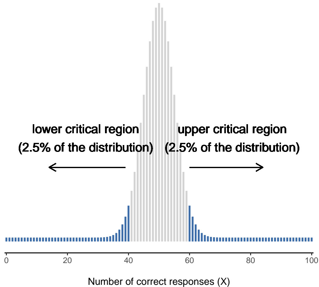
Figure 9.2: The critical region associated with the hypothesis test for the ESP study, for a hypothesis test with a significance level of \alpha = .05 . The plot shows the sampling distribution of X under the null hypothesis (i.e., same as Figure 9.1). The grey bars correspond to those values of X for which we would retain the null hypothesis. The blue (darker shaded) bars show the critical region, those values of X for which we would reject the null. Because the alternative hypothesis is two sided (i.e., allows both \theta < .5 and \theta > .5 ), the critical region covers both tails of the distribution. To ensure an \alpha level of .05 , we need to ensure that each of the two regions encompasses 2.5% of the sampling distribution
