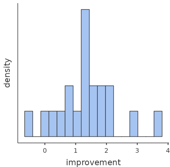
Figure 11.14: Histogram showing the improvement made by each student in Dr Chico's class. Notice that almost the entire distribution is above zero - the vast majority of students did improve their performance from the first test to the second one
