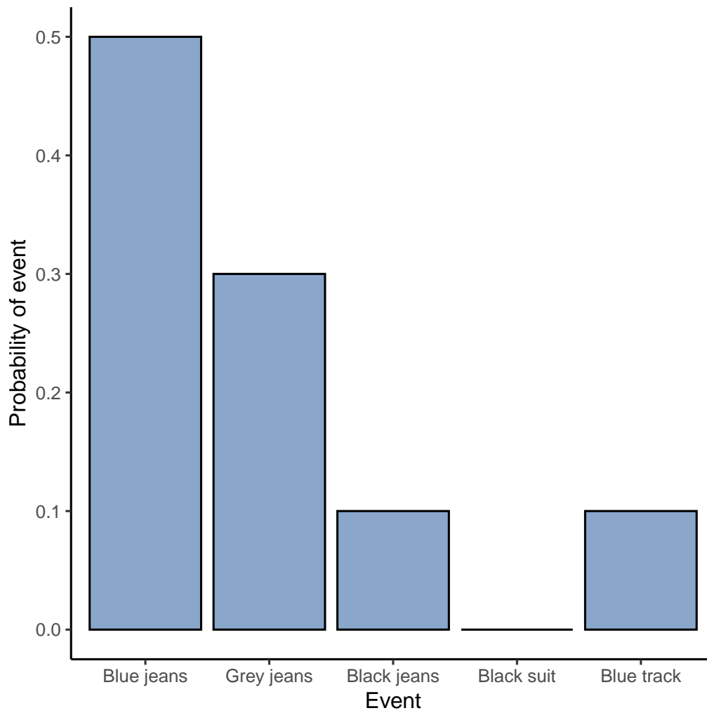
Figure 7.2: A visual depiction of the ‘trousers’ probability distribution. There are five ‘elementary events’, corresponding to the five pairs of trousers that I own. Each event has some probability of occurring - this probability is a number between 0 to 1. The sum of these probabilities is 1
