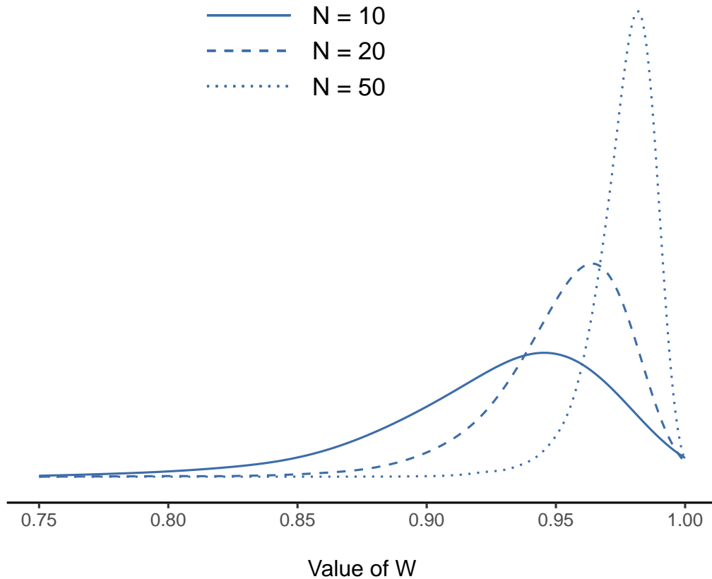
Figure 11.24: Sampling distribution of the Shapiro-Wilk W statistic, under the null hypothesis that the data are normally distributed, for samples of size 10, 20 and 50. Note that small values of W indicate departure from normality
