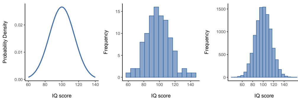
Figure 8.4: The population distribution of IQ scores (panel (a)) and two samples drawn randomly from it. In panel (b) we have a sample of 100 observations, and panel (c) we have a sample of 10,000 observations
