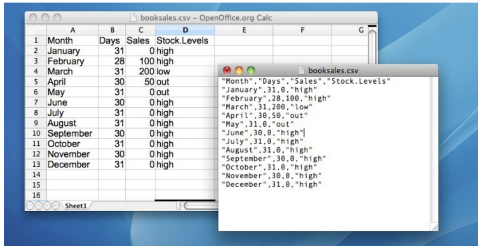
Figure 3.4: The booksales.csv data file. On the left I have opened the file using a spreadsheet program (OpenOffice), which shows that the file is basically a table. On the right the same file is open in a standard text editor (the TextEdit program on a Mac), which shows how the file is formatted. The entries in the table are wrapped in quote marks and separated by commas
